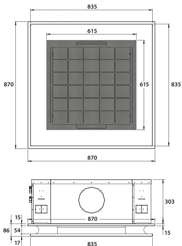
MD800 front
