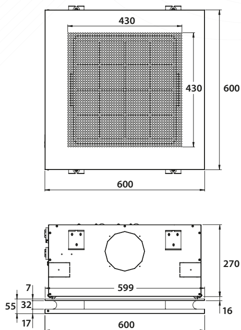
MD600 front
